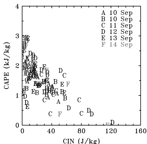
Figure 11. Scatter plots of CAPE and CIN values for the 106 soundings in pre- Karl . Note the tendency for soundings with high values of CAPE to have low values of CIN. This figure is available in colour online at wileyonlinelibrary.com/journal/qj
