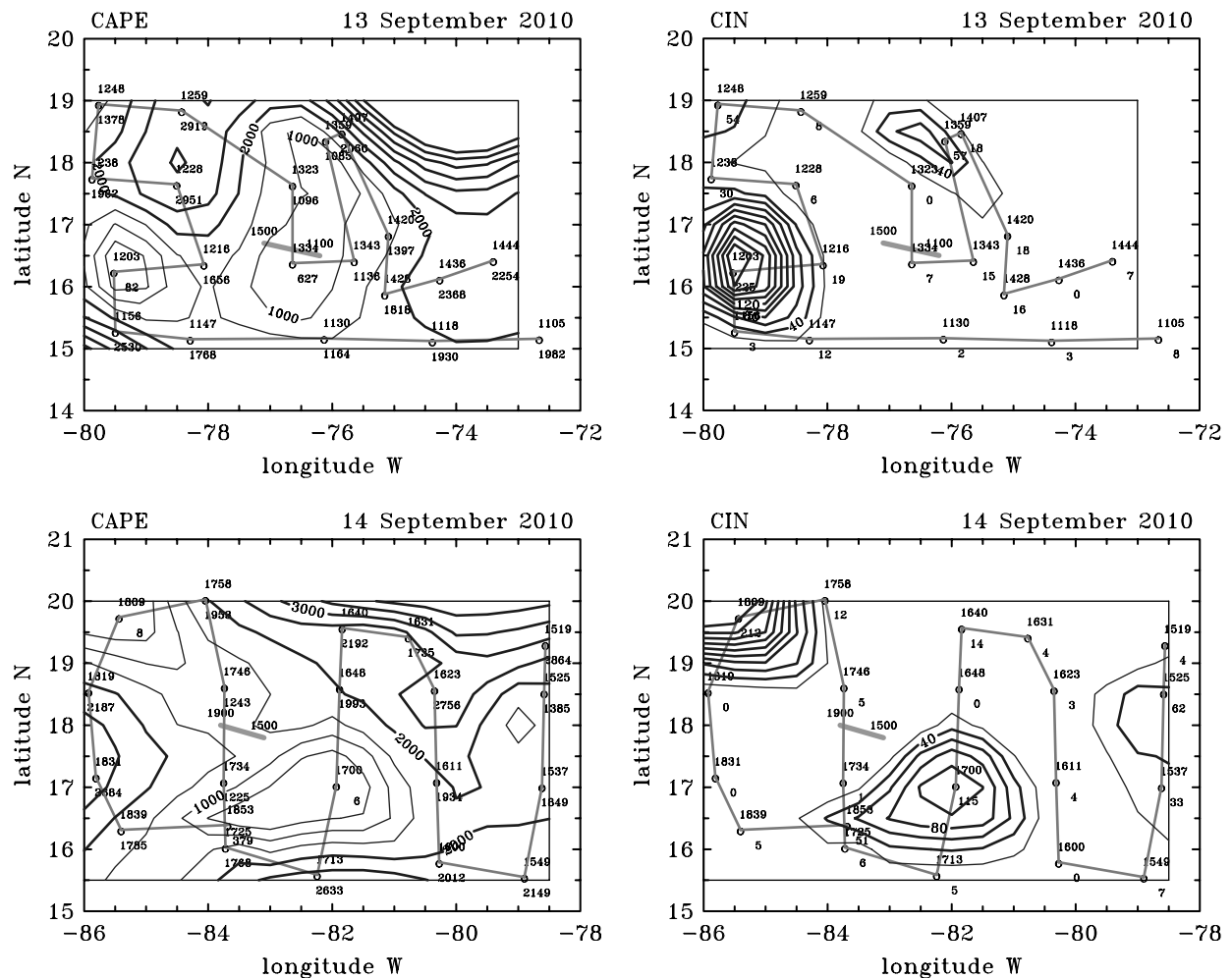
Figure 10. (continued) Objective analyses of CAPE (left columns) and CIN (right columns) for pre-hurricane Karl on 13 and 14 September 2010. This figure is available in colour online at wileyonlinelibrary.com/journal/qj
