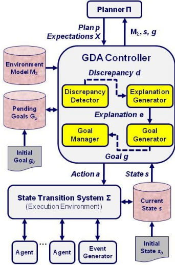
Figure 1: Goal-Driven Autonomy Conceptual Architecture
