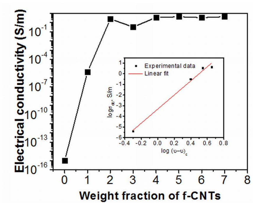
Figure 4: DC electrical conductivity of functionalized carbon nanotubes reinforced PVDF nnaocomposites.
