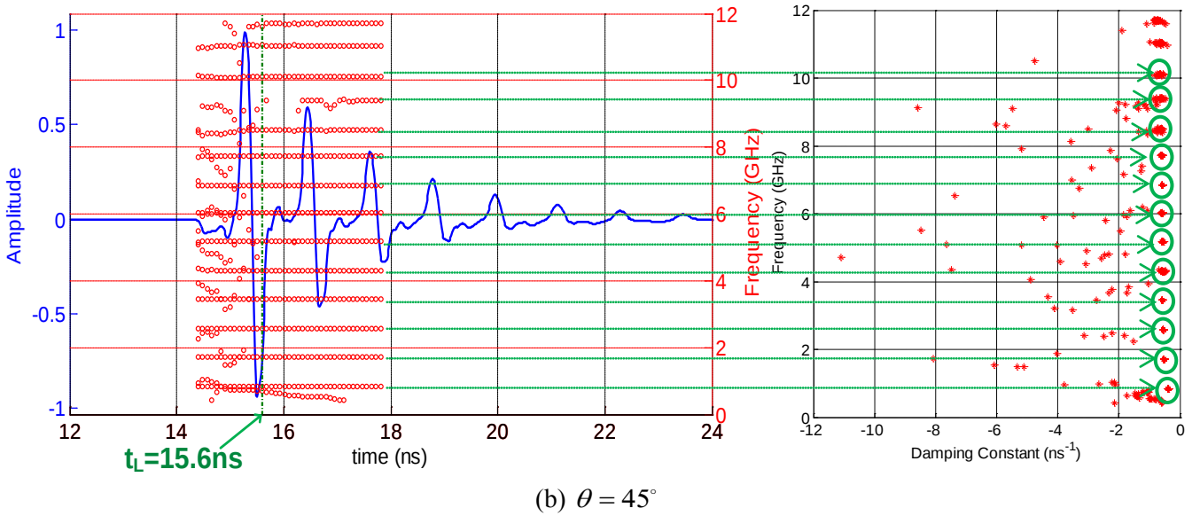
Figure 5. Estimated poles from the wire backscatter responses. The plots on the left show the poles (frequencies only, no damping constants) estimated at corresponding time window starting points as the window is shifted. The plots on the right show the same poles in the Laplace domain (damping constant vs. frequency). Convergent poles show stability in their values with time window shift.
