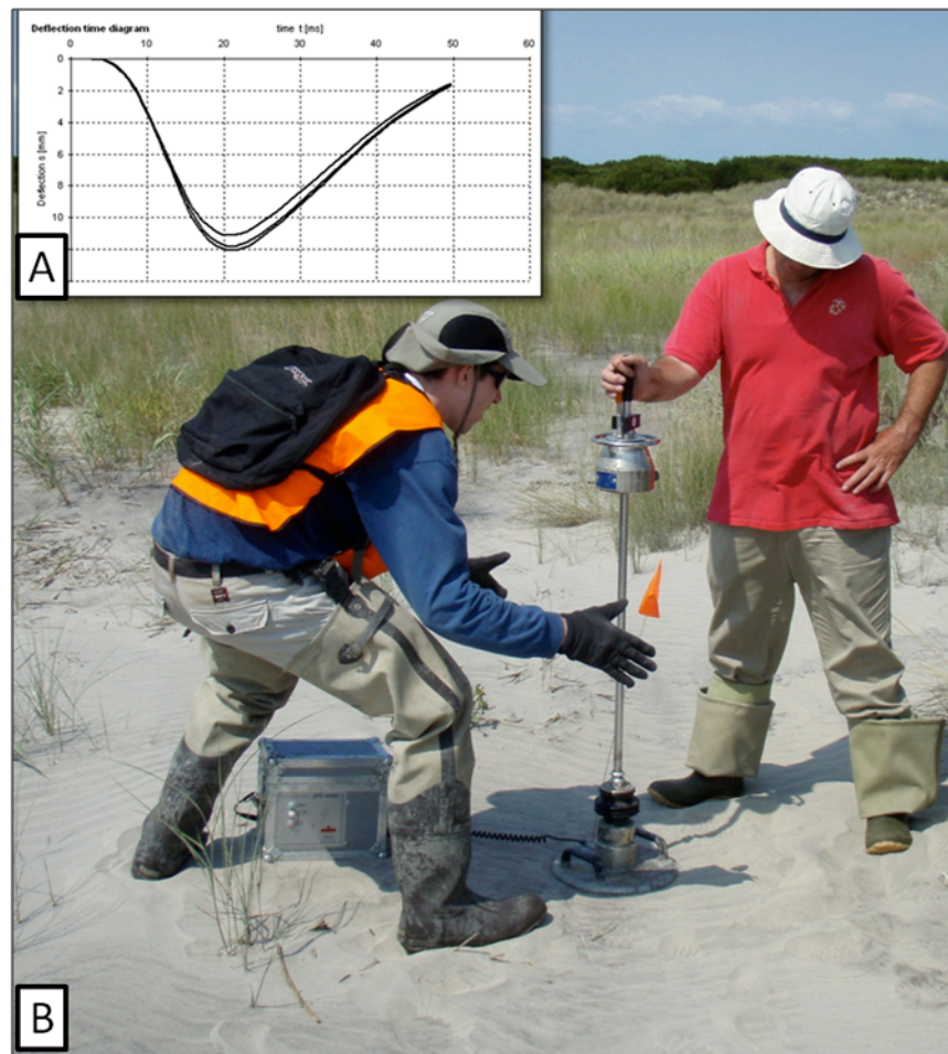
Figure 3.4. The LWD being used to measure dynamic modulus during the VCR'07 campaign. (A)The three pulses showing deflection (mm) as a function of time (ms) used in estimating Evd (B) Light-weight deflectometer (LWD) used to measure dynamic modulus of rigidity, Evd, which is estimated from three successive drops of a 10kg weight along a steel rod attached to a base plate with an embedded accelerometer.
