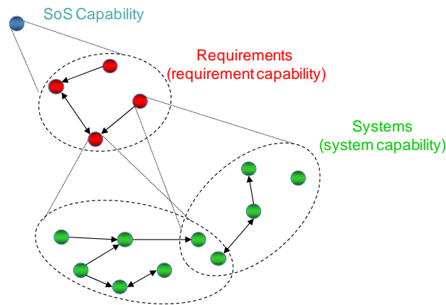
Figure 2. Layered network abstraction of Computational Exploratory Model
