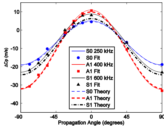
Figure 4.10. Comparison of theory and experiment for an applied uniaxial load of 57.5 MPa at 90° using modified TOECs ( l = -181 GPa, m = -289 GPa, and n = -336 GPa).
