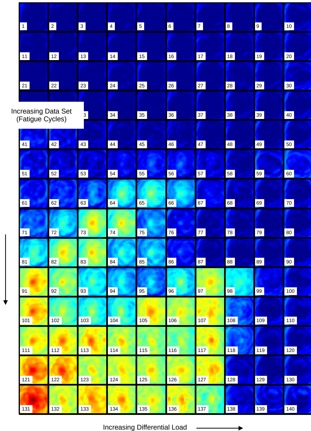
Figure 6.8. Load-differential images of the first 14 data sets from Plate #5 plotted on a fixed 30 dB scale normalized to the overall peak amplitude (-21 to +9 dB).
