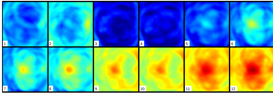
Figure 6.24. Composite load-differential images from all 12 data sets of Plate #7. All images are shown on the same 20 dB color scale (-18 dB to +2 dB).
