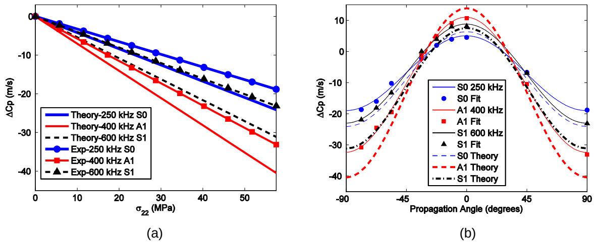
Figure 4.9. Comparison of theory and experiment for propagation in aluminum for a uniaxial load at 90°. (a) Changes in phase velocity versus load for waves propagating at an angle of 90°, and (b) changes in phase velocity versus propagation angle for an applied load of 57.5 MPa.
