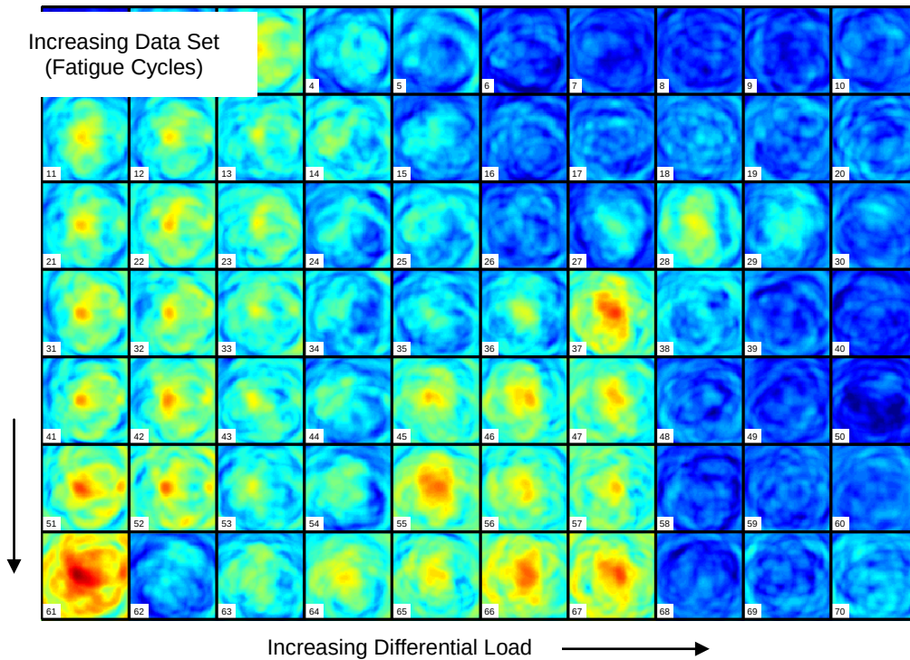
Figure 6.13. Load-differential images of the final seven data sets from Plate #3 with transducer pair 5-6 removed and plotted on a fixed 20 dB scale (-11 to +9 dB).
