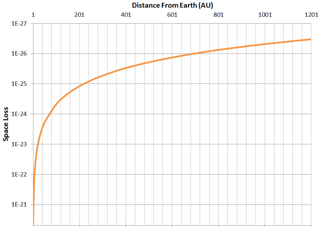
Figure 3.3: Space Loss
