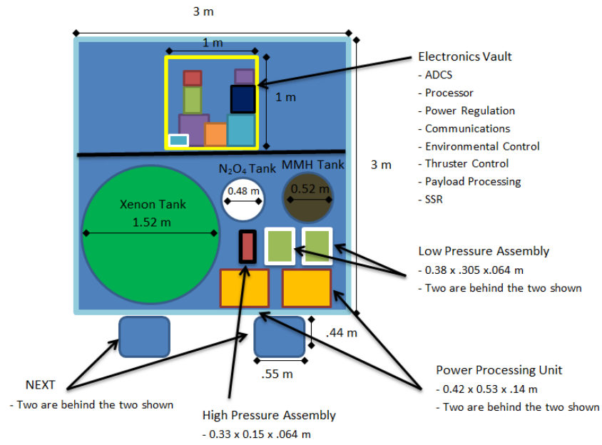
Figure 4.8: Internal Configuration
