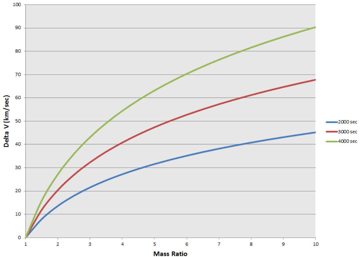
Figure 3.2: Effect of Specific Impulse on \Delta V
