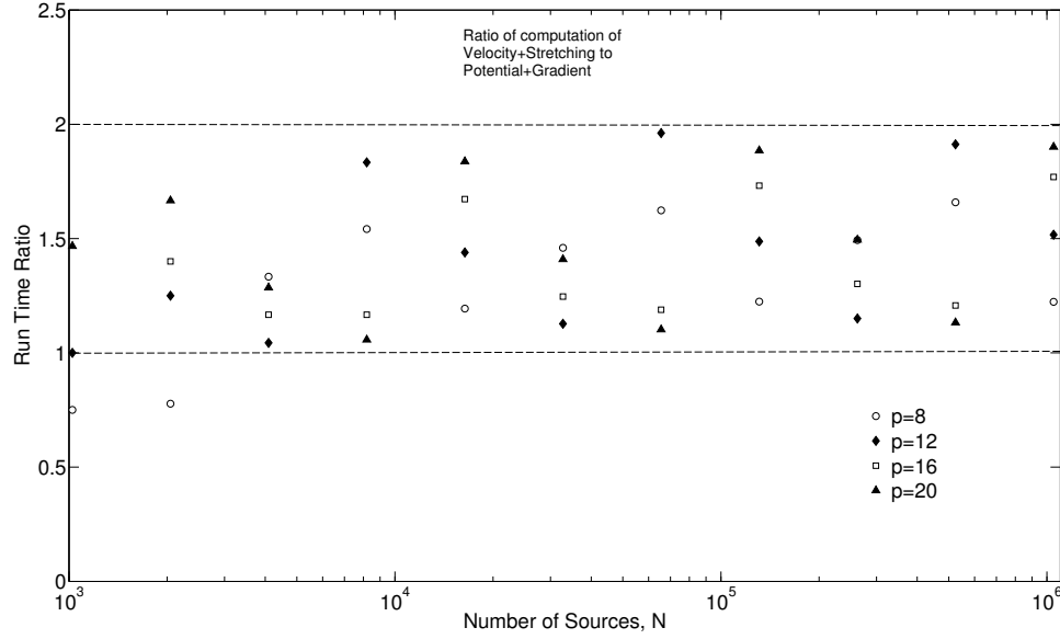
Figure 3: The ratio of the FMM run time for computation of the velocity and stretching term in a vortical flow to the respective time for the potential and gradient computations in a potential flow for different truncation numbers p and number of sources, N , which were randomly and uniformly distributed inside a cube. All data for N > 2048 are located between the dashed lines.
