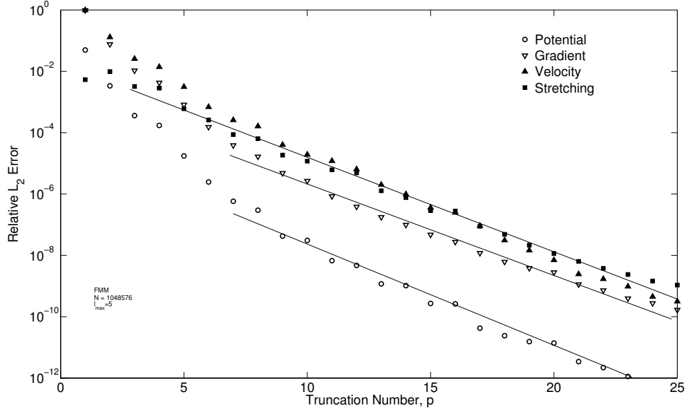
Figure 1: Dependences of the relative FMM errors in the L_2 norm on the truncation number, p . Errors were computed over 1000 random points for N = 2^{20} sources of random intensity distributed uniformly randomly inside a cube. The maximum level of space subdivision l_{\max} = 5 .
