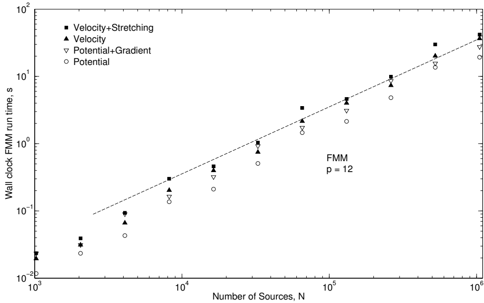
Figure 2: The wall clock time for the FMM for computation of vortical and potential flows (different terms and combinations). The straight line shows linear dependence. For all cases the sources are distributed randomly and uniformly inside a cube; the truncation number is constant, p = 12 .
