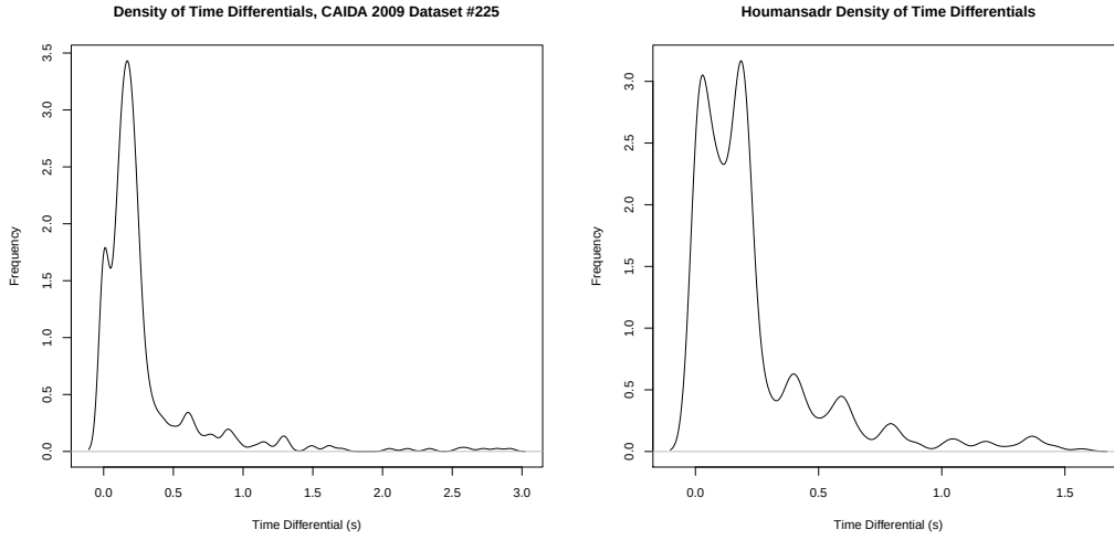
(a) Density of Inter-packet Delays, Sample 225 (b) Density of Houmansadr Data, Sample 4
