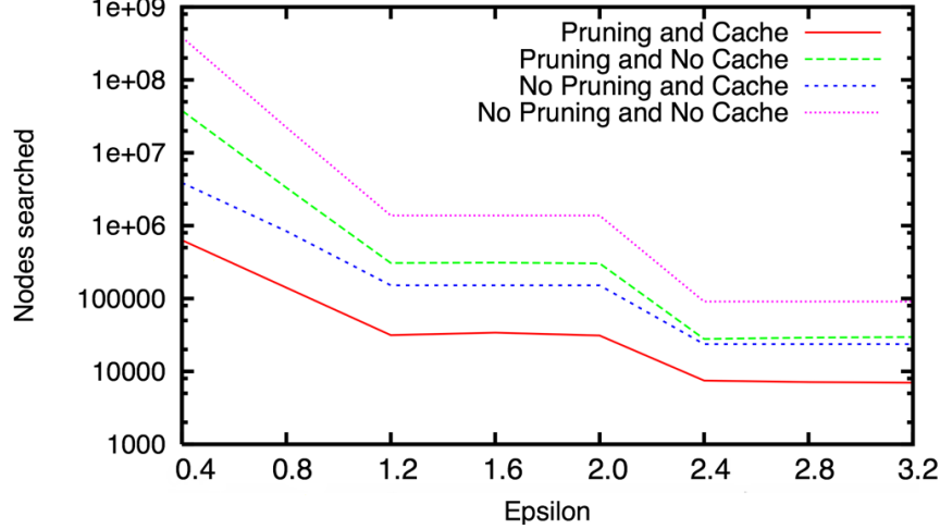
Figure 2: Number of nodes searched in the uniform1 environment, with different combinations of caching and pruning.
