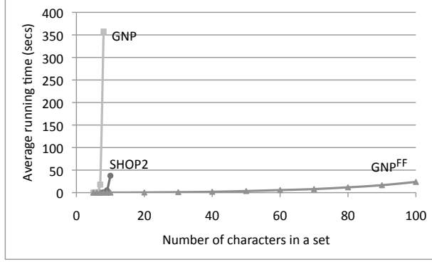
Figure 6: Average running times of SHOP2, GNP, and \text{GNP}^{FF} in 3-Set Character Sequencing, as a function of number of characters per set. Each data point is an average of 100 problems.
