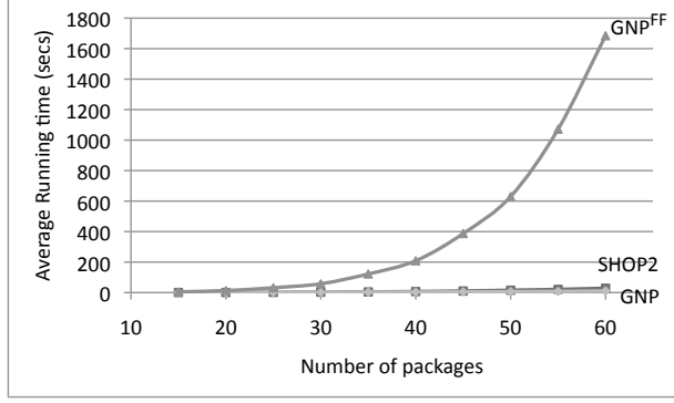
Figure 2: Average running times of SHOP2, GNP, and \text{GNP}^{FF} in the Logistics domain, as a function of the number of packages. Each data point is an average of 100 problems.
