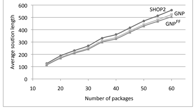
Figure 3: Average length of solutions generated by SHOP2, GNP, and \text{GNP}^{FF} in the Logistics domain, as a function of the number of packages, on the problems in Fig. 2.
