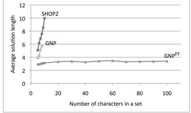
Figure 7: Average length of solutions generated by SHOP2, GNP, and \text{GNP}^{FF} in 3-Set Character Sequencing, as a function of the number of characters per set, on the problems in Fig. 6.
