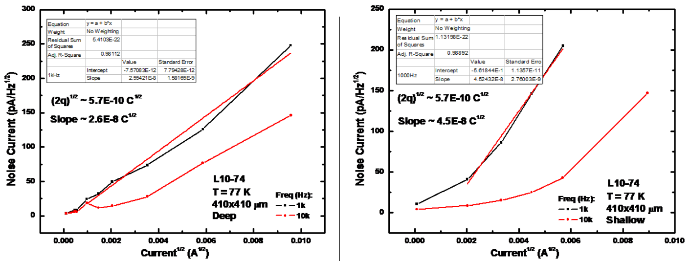
Figure 8. Further illustration of 1/f noise in deep (left), and shallow (right) etched nBn detectors
