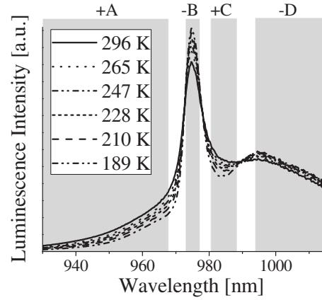
FIG. 5. ^2F_{5/2} \rightarrow ^2F_{7/2} luminescence spectra of \text{Yb}^{3+} in ZBLAN glass at various temperatures. The gray areas indicate wavelength regions in which the luminescence intensity increases (A and C) and regions where the luminescence intensity decreases (B and D) as the temperature is raised. Portions of regions A and D can be selected with commercially available interference filters.
