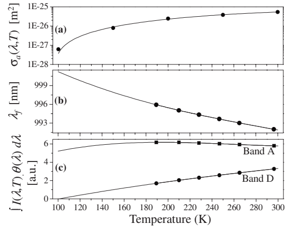
FIG. 6. Temperature dependence of spectroscopic parameters of ZBLAN: \text{Yb}^{3+} : (a) absorption cross section \sigma_a(\lambda, T) at \lambda_p=1020.6 nm (Ref. 26), (b) mean luminescence wavelength \bar{\lambda}_f derived from luminescence spectra at different temperatures, and (c) spectral overlap integrals \int I(\lambda, T) \theta_A(\lambda) d\lambda (circles) and \int I(\lambda, T) \theta_D(\lambda) d\lambda (squares) [see Eq. (18)]. The solid lines in each of the plots are least-squares fits to a cubic polynomial, and the respective parameters are summarized in Table I.
