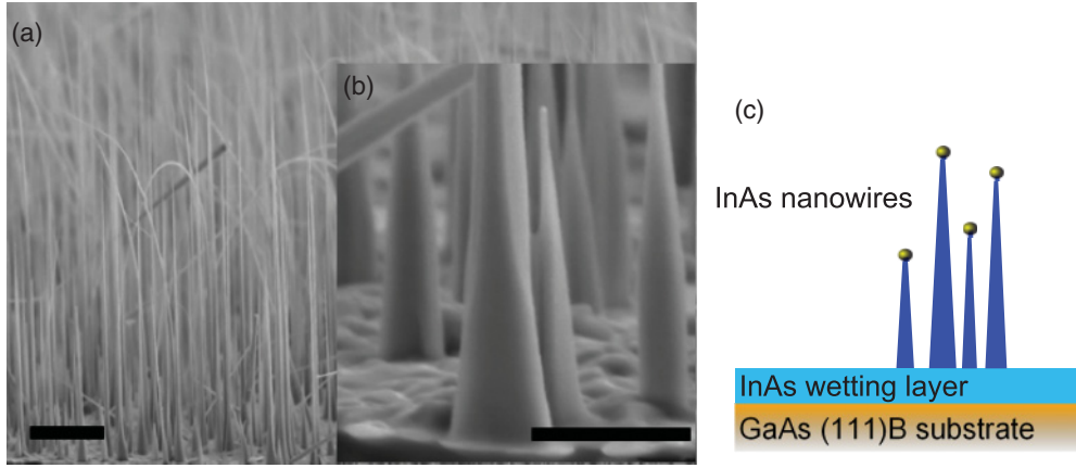
FIG. 1. (Color online) (a) Low-magnification cross-sectional SEM image of the InAs nanowire ensemble, highlighting the nanowires' high aspect ratio and their taper. The scale bar is 3\ \mu\text{m} across. (b) Higher-magnification SEM image showing the base dimension and existence of a planar wetting layer formed by vapor–solid epitaxy. The scale bar is 1\ \mu\text{m} across. (c) Sketch (not to scale) of the three regions of the sample that are potential sources of THz radiation transients. Our experiments show that the signal from the InAs nanowires dominates the signal from the InAs wetting layer or the Si-doped GaAs substrate.
