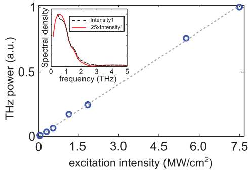
FIG. 3. (Color online) THz power changes linearly as excitation intensity is varied (via a variable neutral density filter) over a range of 150. The inset shows the normalized spectra of THz transients from InAs nanowires as the intensity varies by a factor of 25. Absence of a spectral shift is consistent with radiation emanating from coherent plasma.
