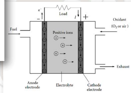
Fuel Cell
