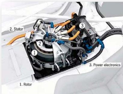
Electric Flywheel
