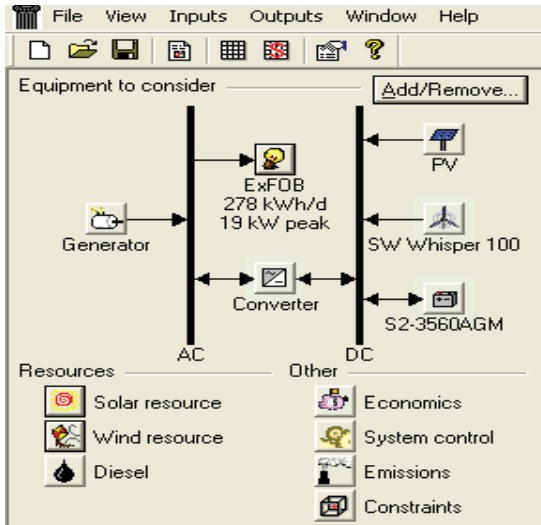
HOMER (National Renewable Energy Laboratory, 2011)
