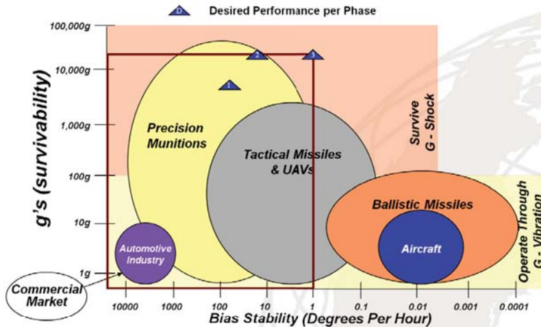
IMU Performance Demands (After Panhorst, et al, 2004)
