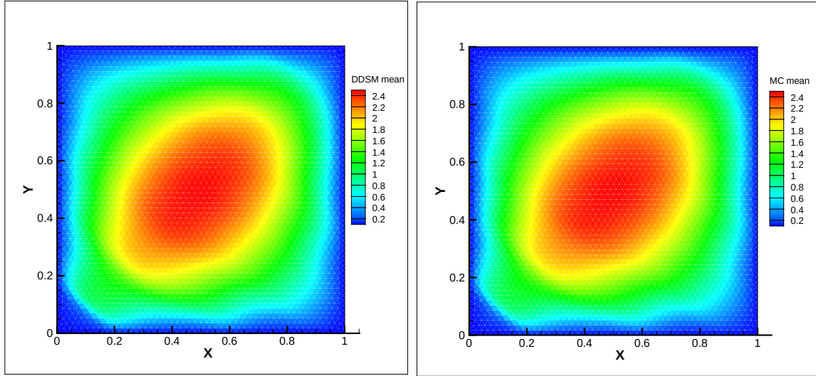
Figure 12: Comparison of mean contour of 2D stochastic Elliptic PDE. Left: adaptive ANOVA-DDSM method using Criterion 3. Right: Monte-Carlo simulation. \Lambda = 1\text{E-}4 and 10 active dimensions.
