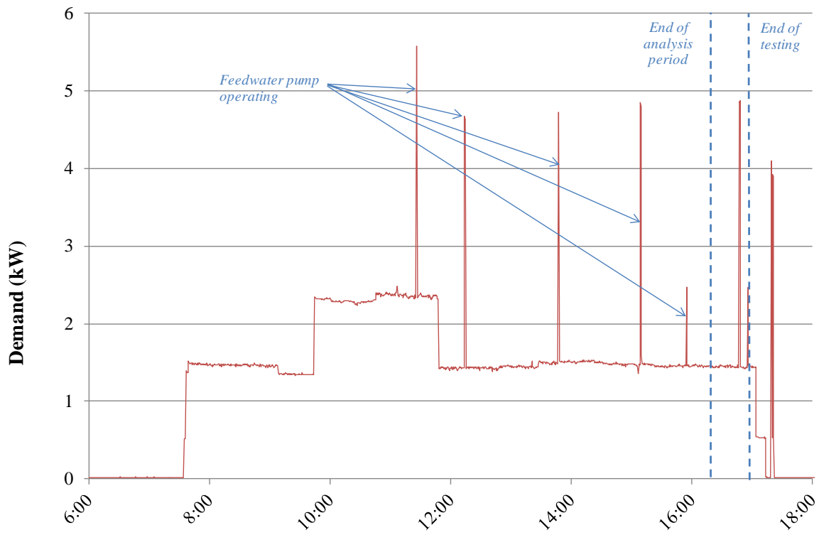
Figure 11. Demand Profile—December 15
