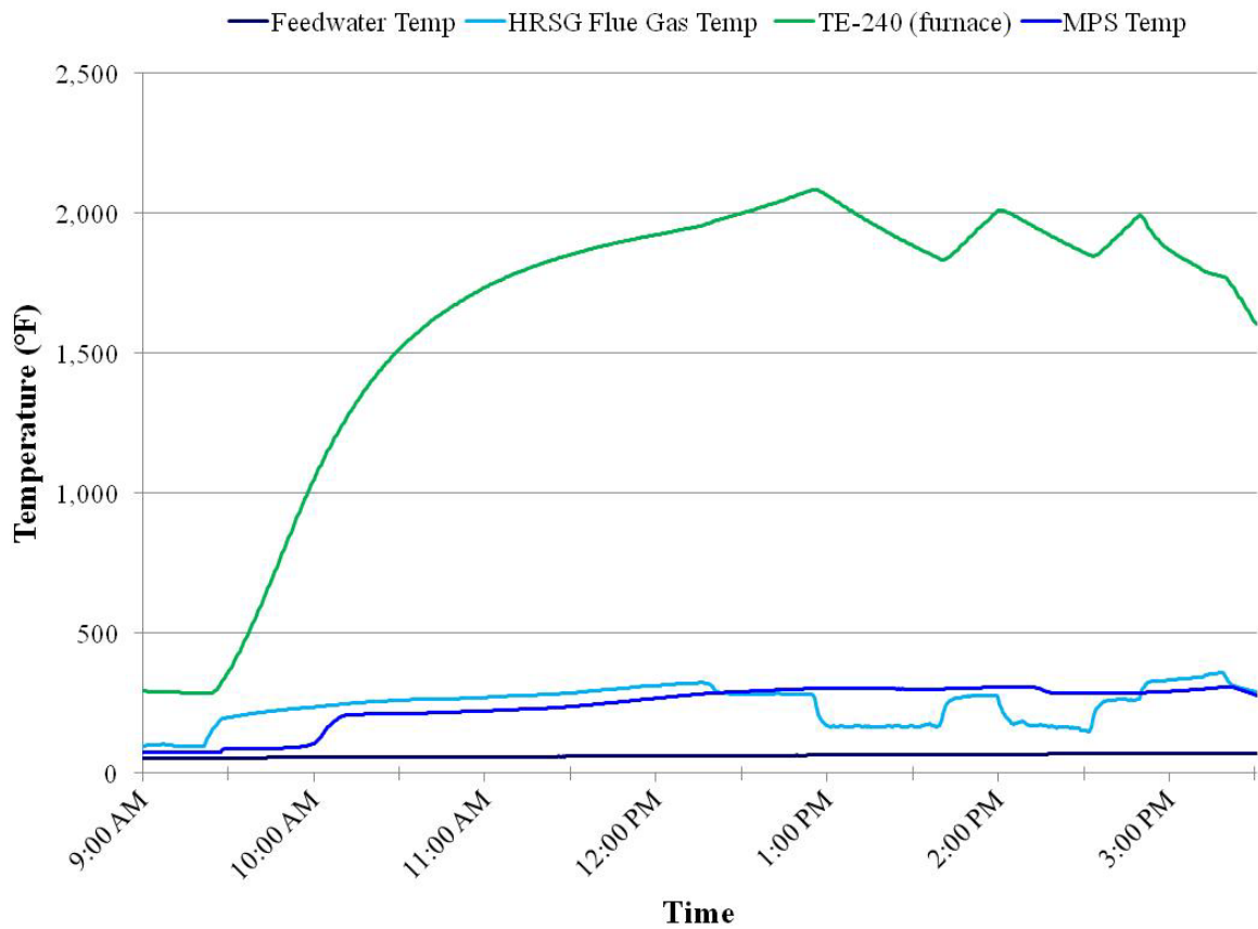
Figure 2. Temperature Profiles during Testing on December 13, 2011
