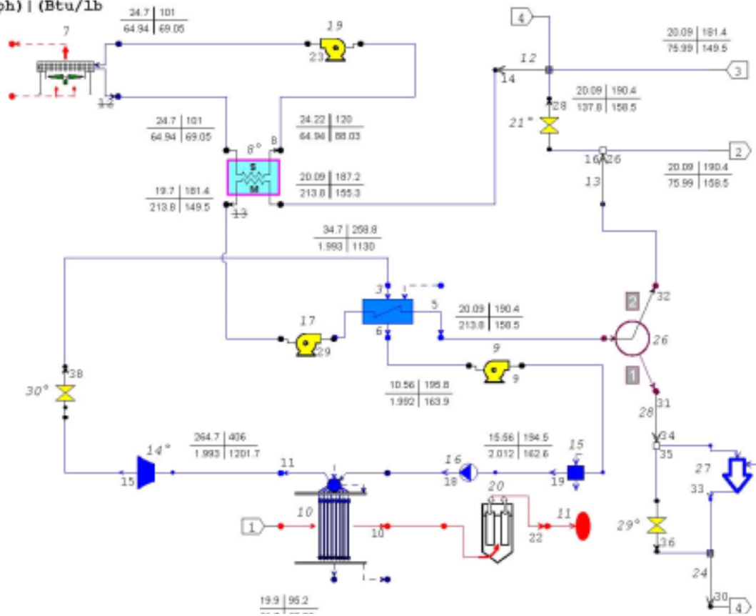
Figure 8. Graphical Heat and Mass Balance—Full Load Biomass Simulation
