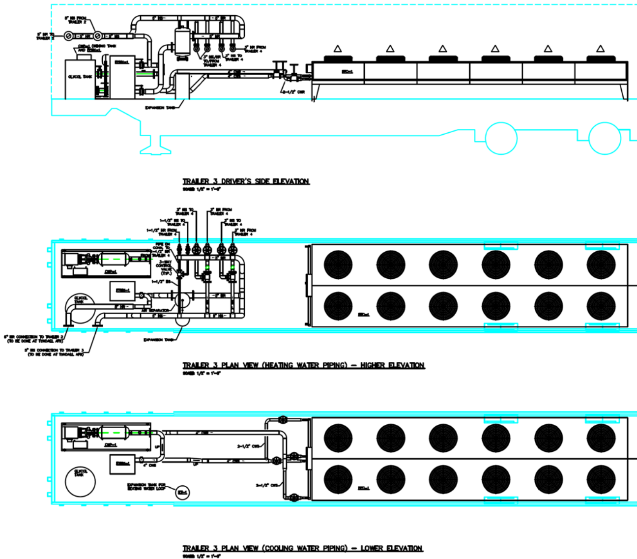
Figure A-2. TWES Trailer 3 Mechanical Plans and Elevations—Phase 1 (Drawing M-3 from 7/27/2009)
