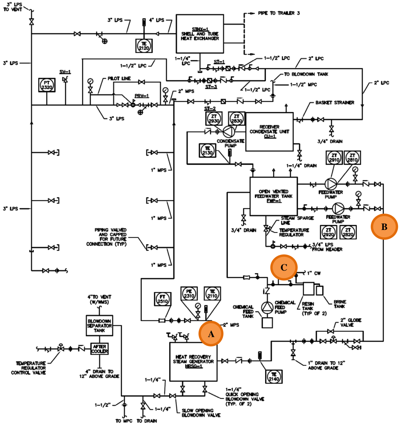
Figure 7. Key State Points
