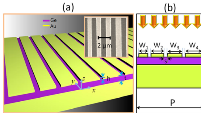
FIG. 6. (a) and (b) Schematic diagram of the proposed three-layered light harvesting absorber. The inset of (a) shows the SEM image of the fabricated sample with P=6.06 \mu\text{m} , t=340 \text{ nm} , and h=16.5 \text{ nm} . Strip widths
