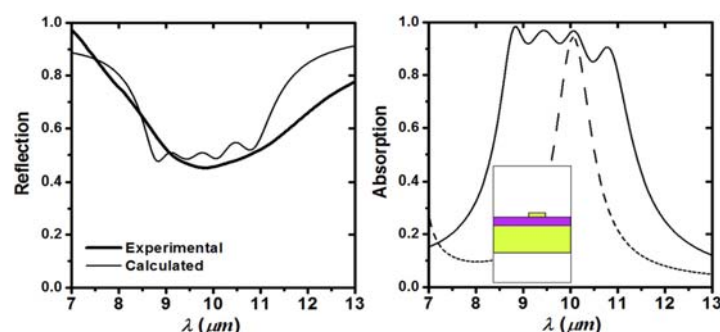
FIG. 7. (a) The experimental (thick curve) and simulated (thin curve) reflection spectra. (b) Comparison of the calculated absorption spectra between the multi-sized antenna (solid curve) and the single-sized antenna absorbers (dashed curve, with the profile shown in the inset).
