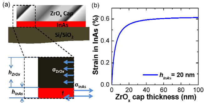
FIG. 4. (Color online) (a) Schematic of the stress distribution across a cross-section of \text{ZrO}_x cap and InAs layer. \sigma_{\text{ZrO}_x} and \sigma_{\text{InAs}} are the normal stresses in \text{ZrO}_x and InAs, respectively, f is the force applied to the InAs layer from the substrate to neutralize the total force. (b) The dependence of the strain ( \epsilon ) in the InAs XOI layer ( h_{\text{InAs}}=20 nm) on the \text{ZrO}_x cap thickness ( h_{\text{ZrO}_x} ).
