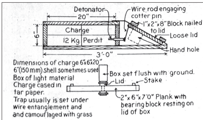
Ingenious Tripping Device for German Trap Mine
