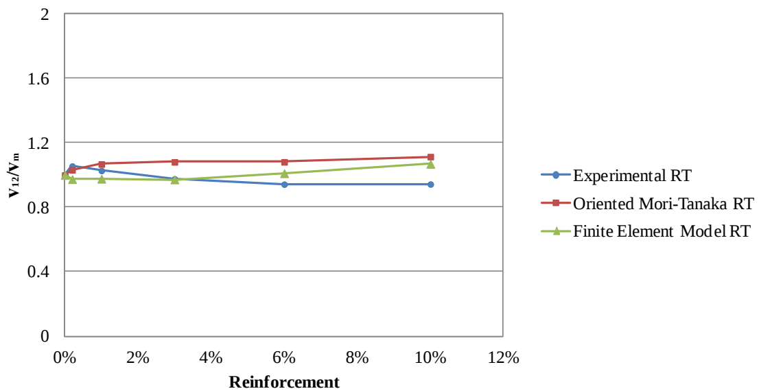
Figure 28. Comparison of v_{12}/v_m values obtained from the experimentally, Mori-Tanaka calculation and the finite element model at room temperature
