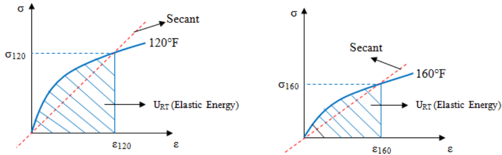
Figure 19. Calculation of secant Young's modulus from nonlinear material curve at (a) 120°F and (b) 160°F
