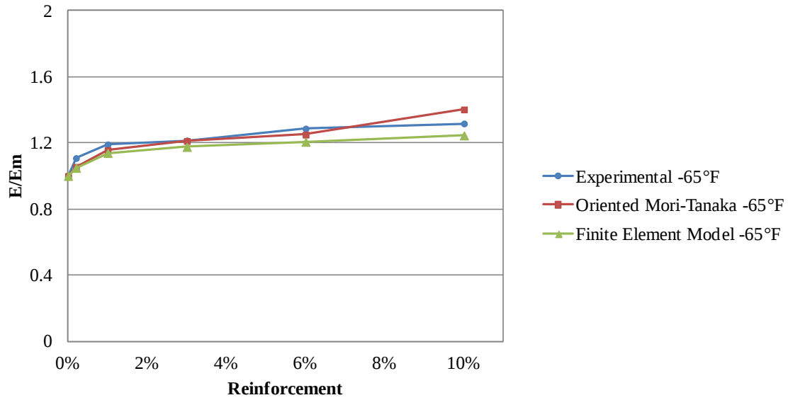
Figure 23. Comparison of E/E_m values obtained from the experiments, Mori-Tanaka calculations and the finite element model at -65°F
