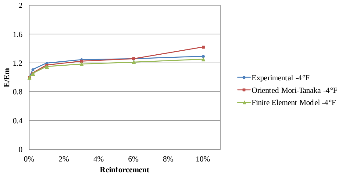
Figure 24. Comparison of E/E_m values obtained from the experiments, Mori-Tanaka calculations and the finite element model at -4°F
