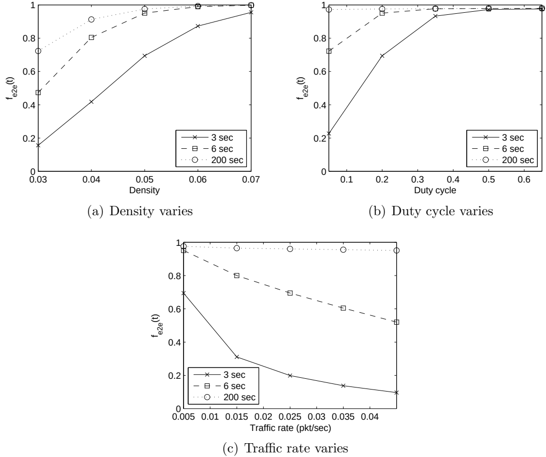
Figure 3.13: The relationship between network parameters and the delivery probability with the Anycast protocol.
