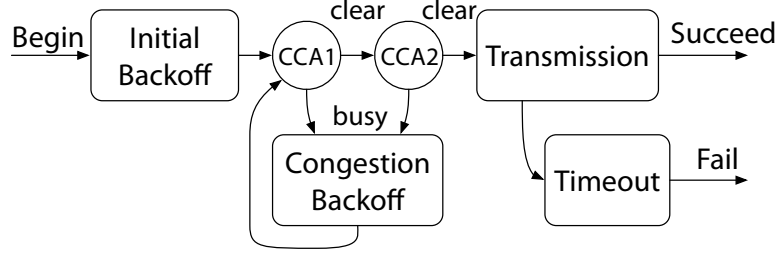
Figure 3.5: The transmission process for a packet with the TinyOS CSMA/CA MAC protocol. Figure 2.2 is redrawn here for convenience.
