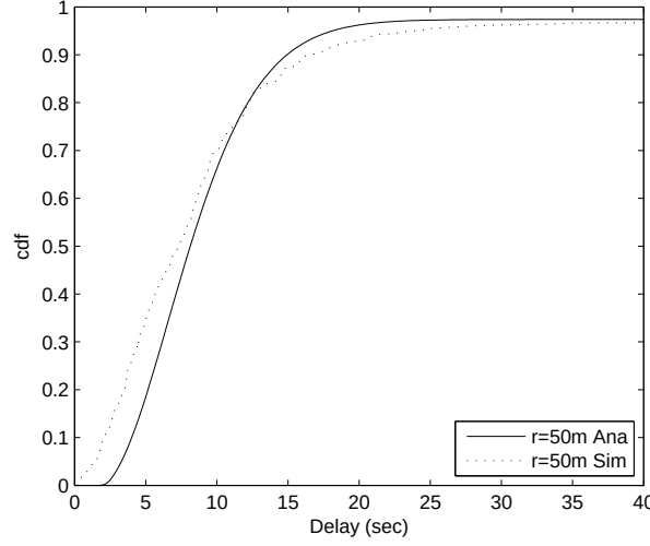
Figure 3.12: The analysis and simulation results of end-to-end delay distribution with the Anycast protocol for a node with distance r = 50 m to the sink.
