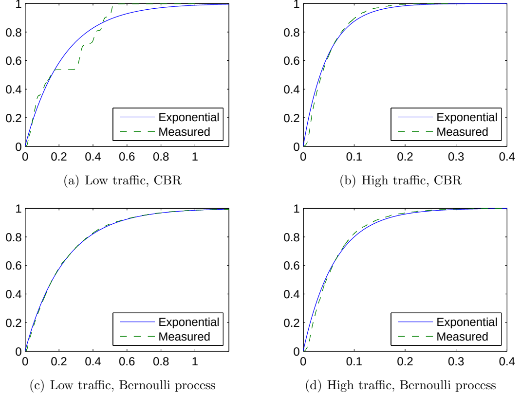
Figure 2.1: The distribution of inter-arrival time for different types of traffic in a 10-hop chain network.
