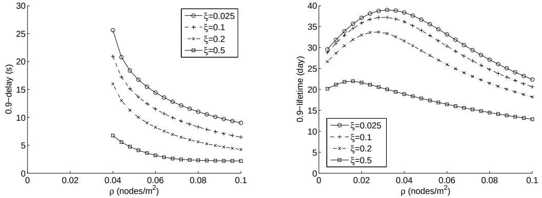
(a) 0.9-quantile of the end-to-end delay vs. network density. Traffic rate is fixed as 0.008 pkt/s. (b) 0.9-quantile of the network lifetime vs. network density. Traffic rate is fixed as 0.008 pkt/s.
