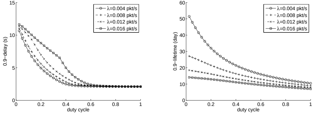
(a) 0.9-quantile of the end-to-end delay vs. duty cycle. Network density is fixed as 0.08 nodes/m 2 . (b) 0.9-quantile of the network lifetime vs. duty cycle. Network density is fixed as 0.08 nodes/m 2 .
