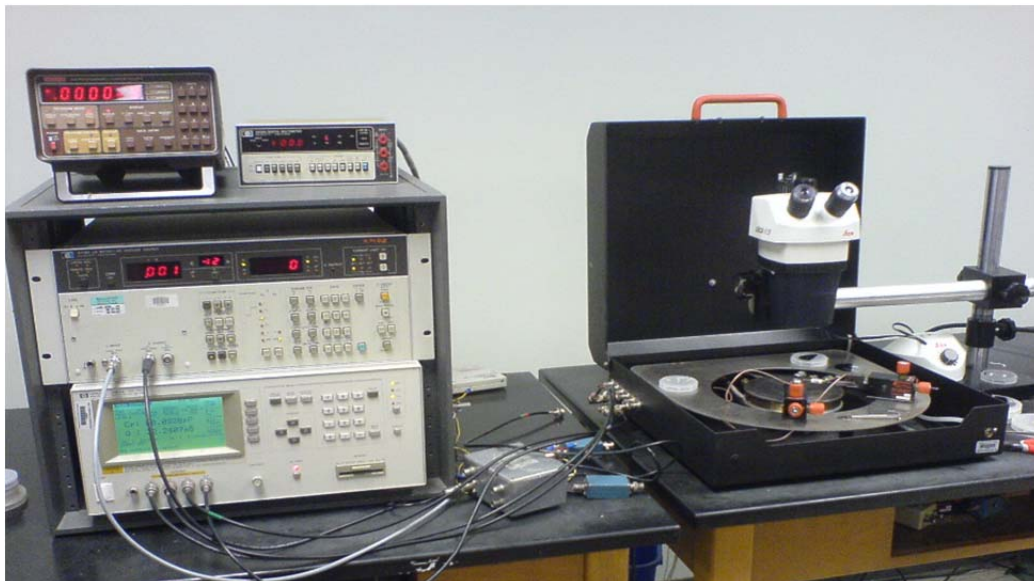
Figure 3. MOS measurement station at the University of Houston.
