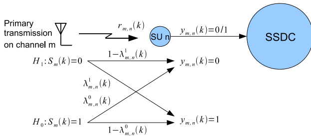
Fig. 2. SUs' reports of observations on primary channels can be modeled as Binary Asymmetric Channels.
