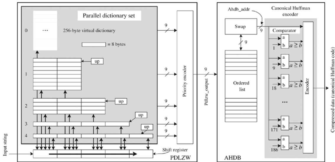
Figure 35. Hardware proposal of Parallel Dictionary LZW plus adaptive Huffman showing the four variable-length dictionaries on the left for word lengths from five to two, and the adaptive Huffman priority queue on right (From [27]).
