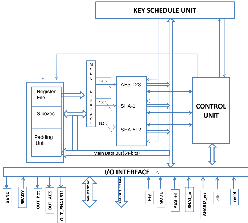
Figure 50. Main architecture of HSSec cryptographic coprocessor (From [62]). The control unit manages data processing and communication with the outside world. Cryptographic primitives (AES-128, SHA-1, and SHA-512) are arranged in a parallel orientation and use a common 64-bit global data bus. The key-scheduler block is used for key expansion and generating message schedules. The memory block consists of a register file, padding unit, and S boxes. The mode interface is responsible for modifying the input to the cryptographic primitives. The key scheduler performs the RotWord and SubWord transformations described above. The key scheduler also provides constants needed by the hash functions: SHA-1 uses a sequence of eighty, constant 32-bit words, and SHA-512 uses a sequence of eighty, constant 64-bit words.
