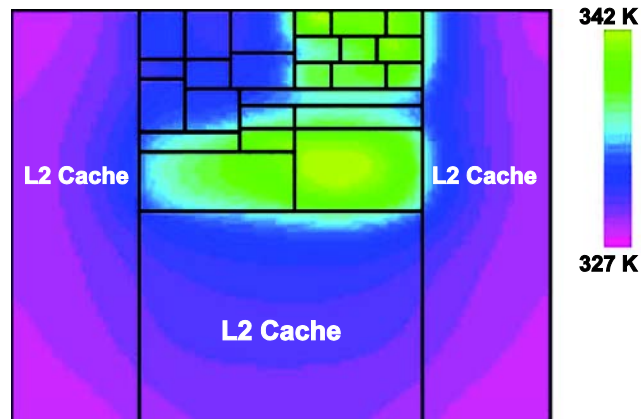
Thermal Profile of the 4-die 3D Processor
