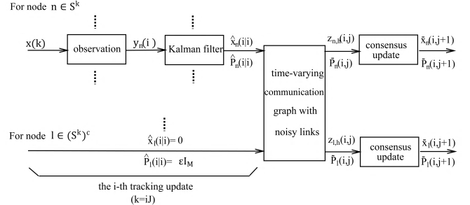
Fig. 2: Block diagram of distributed tracking with consensus on a time-varying graph with incomplete data and noisy communication links.
