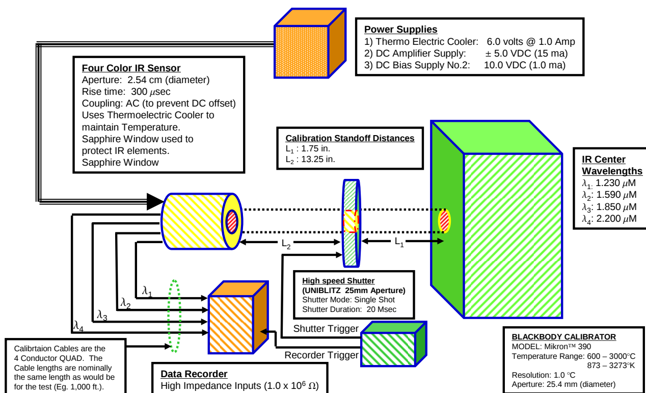
Figure 4, calibration configuration for four color IR.
