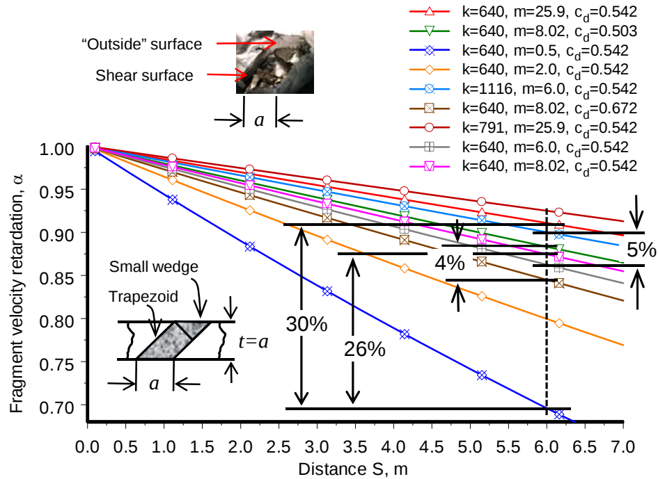
Fig. 4 Fragment velocity retardation factor \alpha versus fragment flight distance S . Fragment shape factors k are \text{grains/in}^3 , fragment masses m are in \text{grains} .
