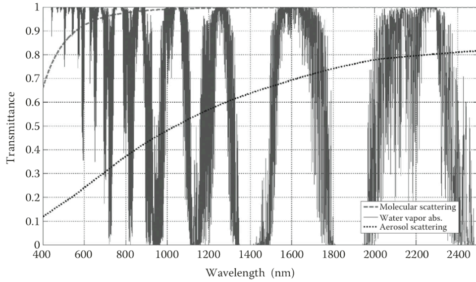
Figure 14. Contribution of Rayleigh scattering, Mie scattering, and water vapor to the atmospheric transmittance (From Hemmati 2009)
