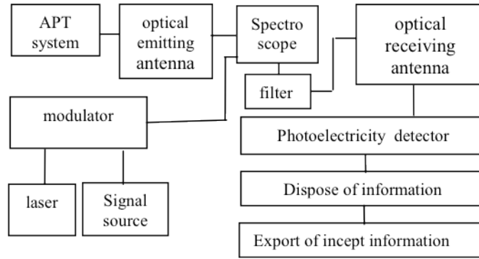
Figure 3. FSOC system (From Li, 2009)
