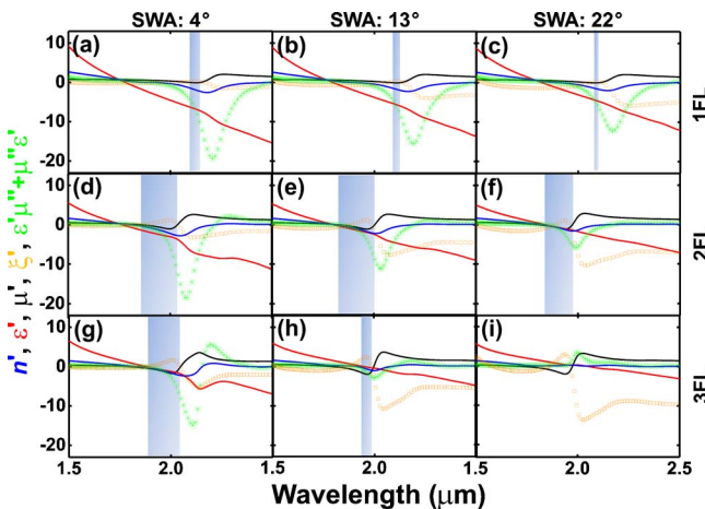
Fig. 4. (Color online) n', \epsilon', \mu', \xi' , necessary condition ( \epsilon' \cdot \mu'' + \mu' \cdot \epsilon'' < 0 ), and sufficient condition ( \epsilon', \mu' < 0 ) for negative refractive index ( n' < 0 ) for one- to three-functional-layered s-eNIMs with sidewall angles (4°, 13°, 22°) are plotted. \xi' has been multiplied by 10 for clarity.
