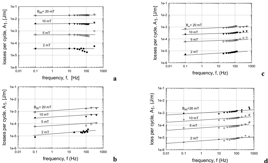
Figure 5. The dependence of losses per cycle on the frequency of the magnetic field at various field amplitudes: a- sample B/0, b – sample B/2, c- sample B/3, d – sample B/4
