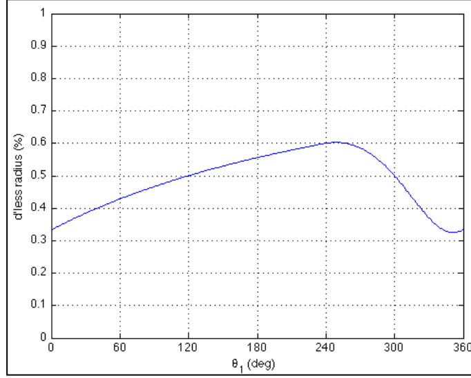
Figure 2. Dimensionless gear radius during one revolution.
