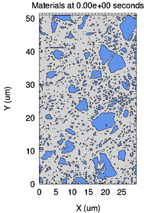
FIG. 7. (Color online) Digitized micrograph taken from Ref. 5. The computed density is 2.496 \text{ g/cm}^3 which corresponds to 48 vol % of epoxy and 52% \text{Al}_2\text{O}_3 .
