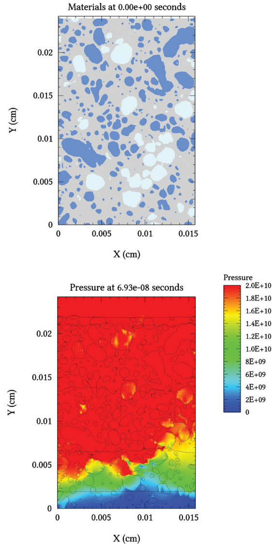
FIG. 8. (Color) Digitized micrograph of Fig. 1(e). The image was rotated 90^\circ to elongate the material in the direction of shock. [ U_{\text{impact}}=450 \text{ m/s} , u_p=332 \text{ m/s} , U_s=2.921 \text{ km/s} , which is shown in Fig. 6(a)]. The pressure distribution is shown at the stage where the shock has almost reached the bottom of the material. The shock-front is nonuniform. The colors correspond to blue=0 GPa, and red=2 GPa. The temperature distribution is shown in the bottom part of the figure. The W particles are clearly distinguished from the soft Al particles, which undergo much more bulk deformation along with the matrix.
