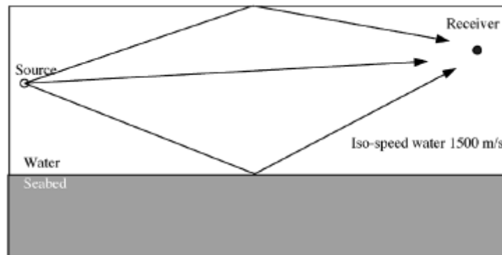
Figure 20. Generalized Pathways of Shock Waves and Sound Energy (adapted from Siderius and Porter, 2006)
