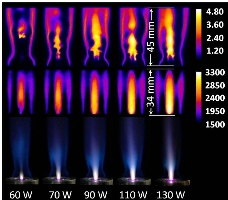
Fig. 2. (Top) Single-shot OH PLIF images, (middle) averaged Rayleigh scattering temperature fields, and (bottom) photographs at total flow rate of 1 LPM of methane and 5 LPM of air for power levels from 60 to 130 W in the non-premixed mode.
