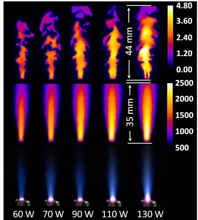
Fig. 1. (Top) Single-shot OH PLIF images, (middle) averaged Rayleigh scattering temperature fields, and (bottom) photographs at a total flow rate of 15 LPM of equivalence ratio of 1.0 for power levels from 60 to 130 W in the premixed mode.
