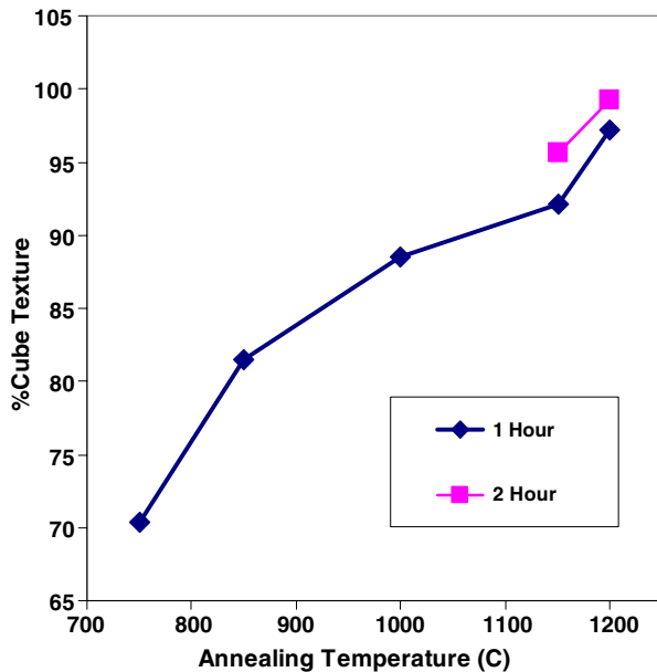
Figure 5. Increase in the percentage cube texture as a function of temperature and time.
