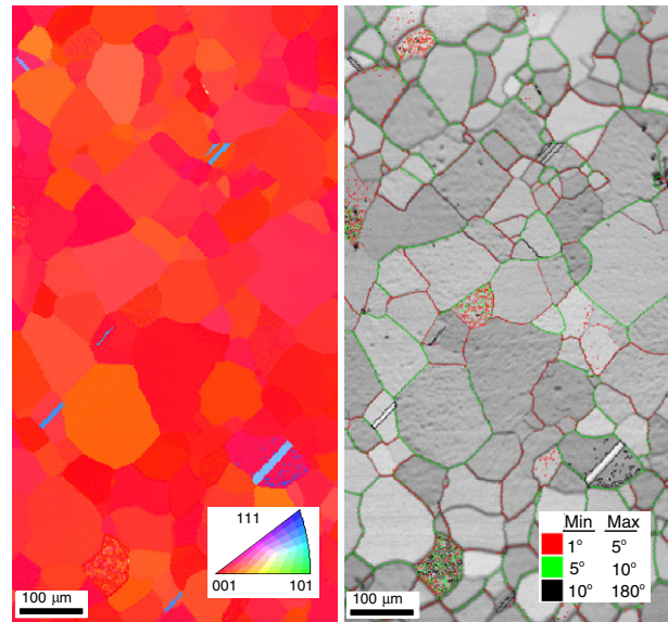
Figure 6. OIM data of a constantan sample annealed at 1200^\circ\text{C} for 2 h.
