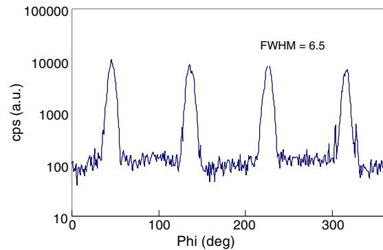
Figure 7. X-ray phi scans (111) of a constantan sample annealed at 1200^\circ\text{C} for 2 h.
