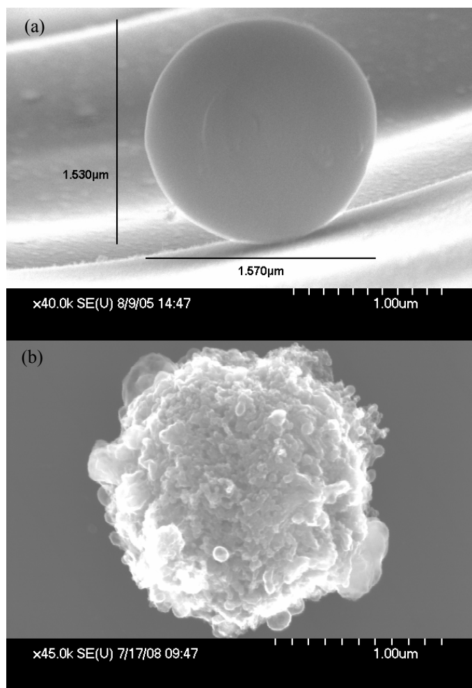
Figure 2. Scanning electron microscope image of a silicon microsphere created by using (a) a cylindrical lens (top) and (b) a similar sized particle created using a spherical lens (bottom).
