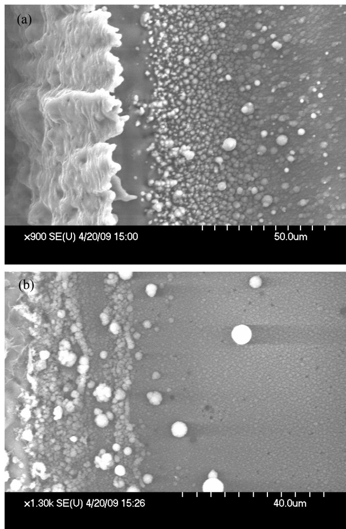
Figure 4. Microspheres formed using an excimer laser energy of (a) 500 mJ and (b) 700 mJ.
