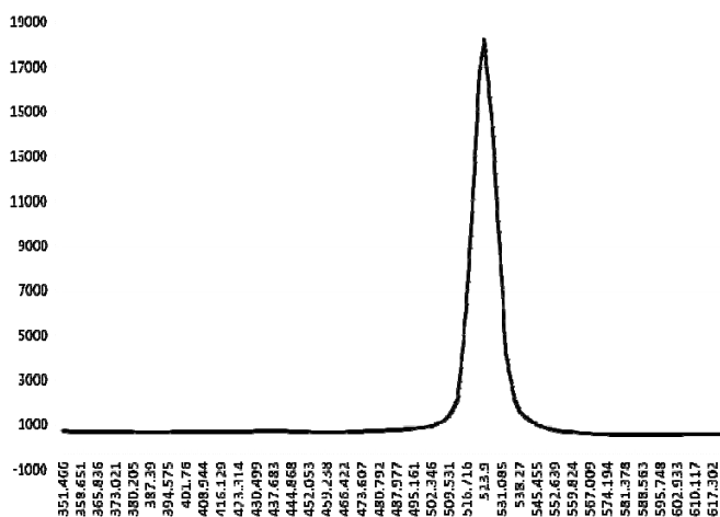
Figure 3. Raman spectroscopy measurements on silicon microspheres. The vertical and horizontal axis represents the 'intensity' (a.u.) and 'Raman shift' ( \text{cm}^{-1} ), respectively.
