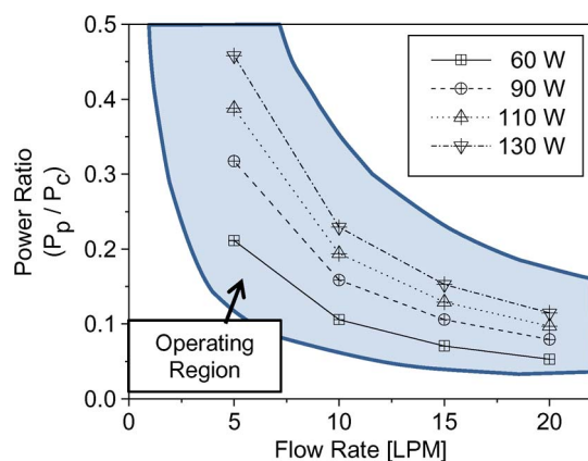
Fig. 1. Plot of the plasma-to-combustion-power ratio the torch operates at. The shaded region shows the total operable region. Flow rate is the total flow rate for a stoichiometric premixed methane/air flame.
