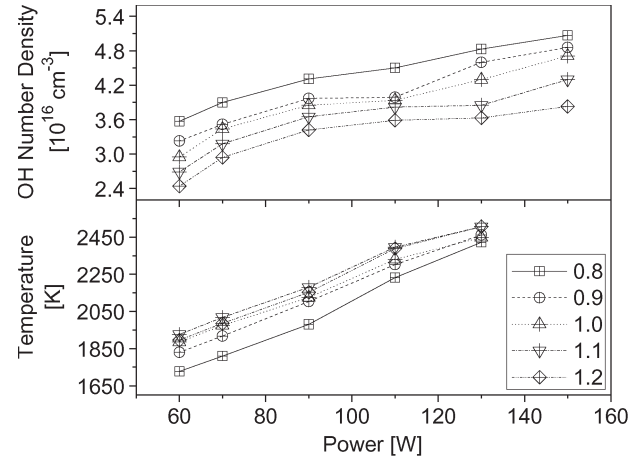
Fig. 7. (Top) OH number density and (bottom) temperature versus power in the premixed plasma discharge for varying equivalence ratios. The total flow rate is 15 l/min.
