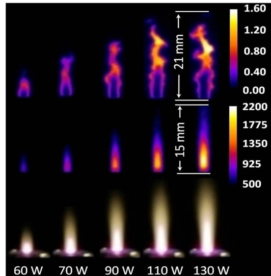
Fig. 3. Images of (top) OH number density [ 10^{16}\text{ cm}^{-3} ], (middle) averaged temperature (in degrees Kelvin), and (bottom) discharge of an air plasma discharge for varying microwave power levels, increasing left to right (15-l/min flow rate).
