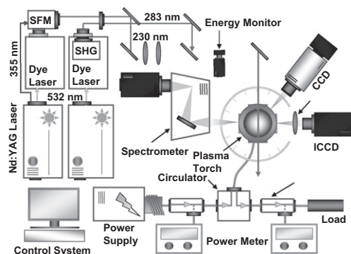
Fig. 2. Experimental setup with bottom part shows microwave energy generation, coupling and monitor system.
