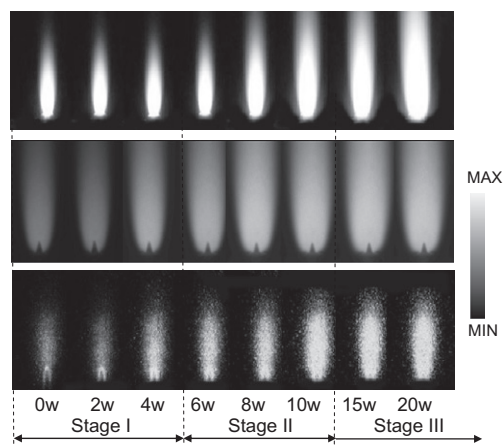
Fig. 3. Emission (top), OH PLIF (middle) and CO PLIF (bottom) intensity images of \text{CH}_4/\text{O}_2 flame vs. microwave power with three stages noted (100 SCCM total flowrate at \phi = 1.1 ).
