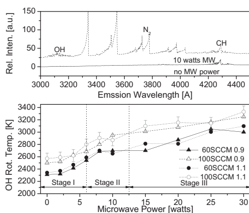
Fig. 6. Emission spectra from CH 4 /O 2 flame with no microwave radiation and 10 W microwave radiation (top) and OH rotational temperature at the same conditions as in Fig. 5 (bottom).
