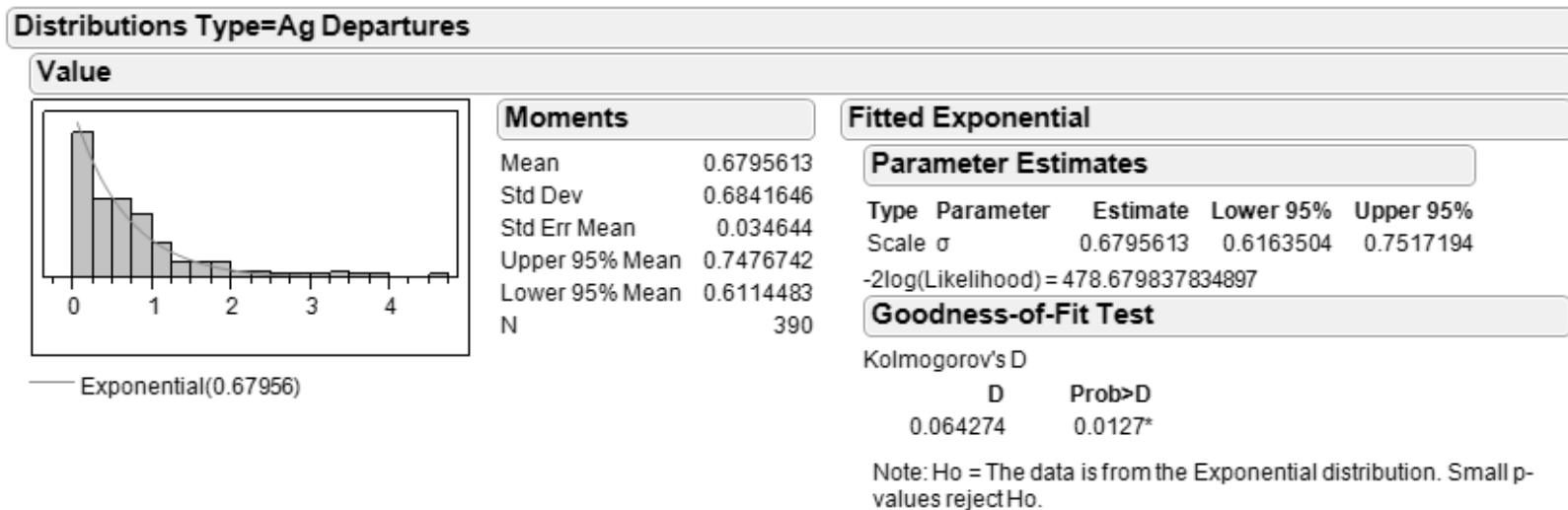
Figure A.9. Sim 5 Distribution Results: D/M/1 Simulation, \hat{\rho}_5 = 0.6708
