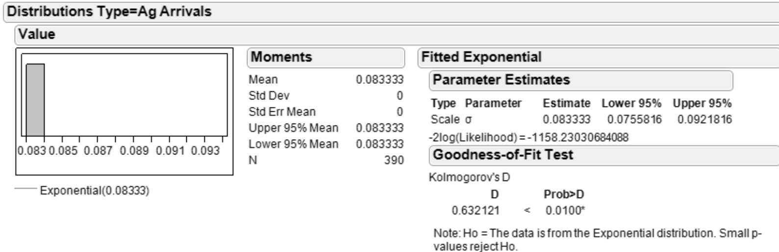
Figure A.9. Sim 5 Distribution Results: D/M/1 Simulation, \hat{\rho}_5 = 0.6708
