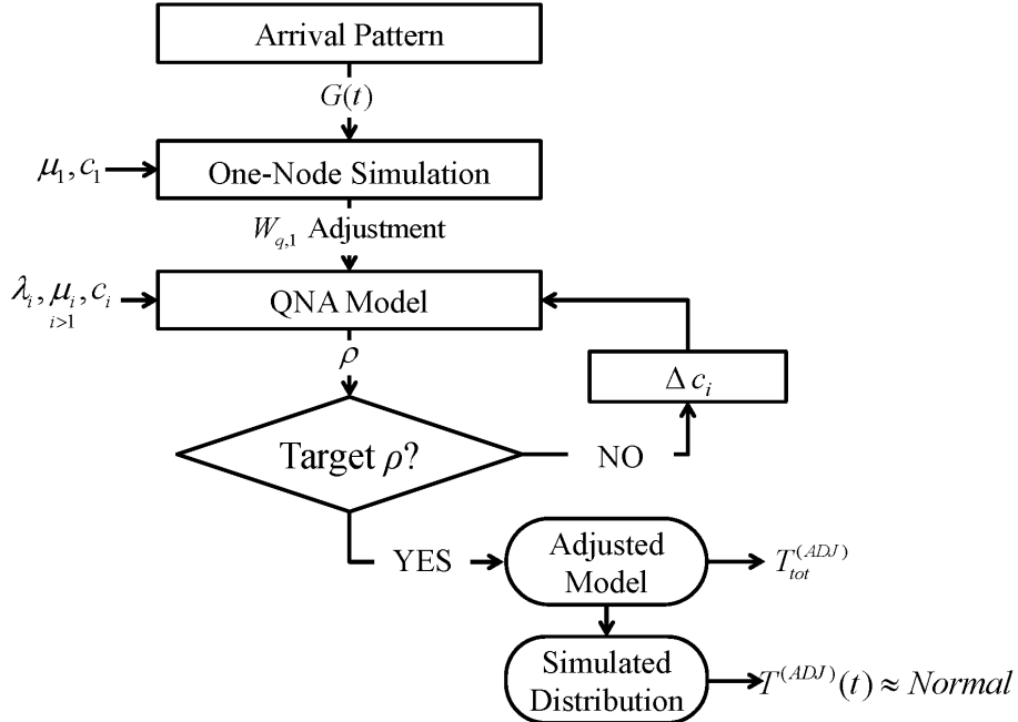
Figure 3.1. Diagram depicting general Sim-QNA hybrid methodology.
