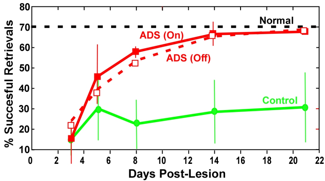
Figure 3. Motor performance on a pellet retrieval task in rats after controlled cortical impact in the primary motor cortex (CFA). Uninjured rats (Normal; n=6 ) perform at \sim 70\% success (from Nishibe et al., 2010). Impacted, but untreated rats ( n=3 ) perform at 20-30% success. This level is similar to that seen in our previous full report of untreated rats (Nishibe et al., 2010). Rats with activity-dependent stimulation (ADS) recover rapidly, and are indistinguishable from normal rats by post-lesion day 14. Data for the ADS group is collected with the microdevice ON.
