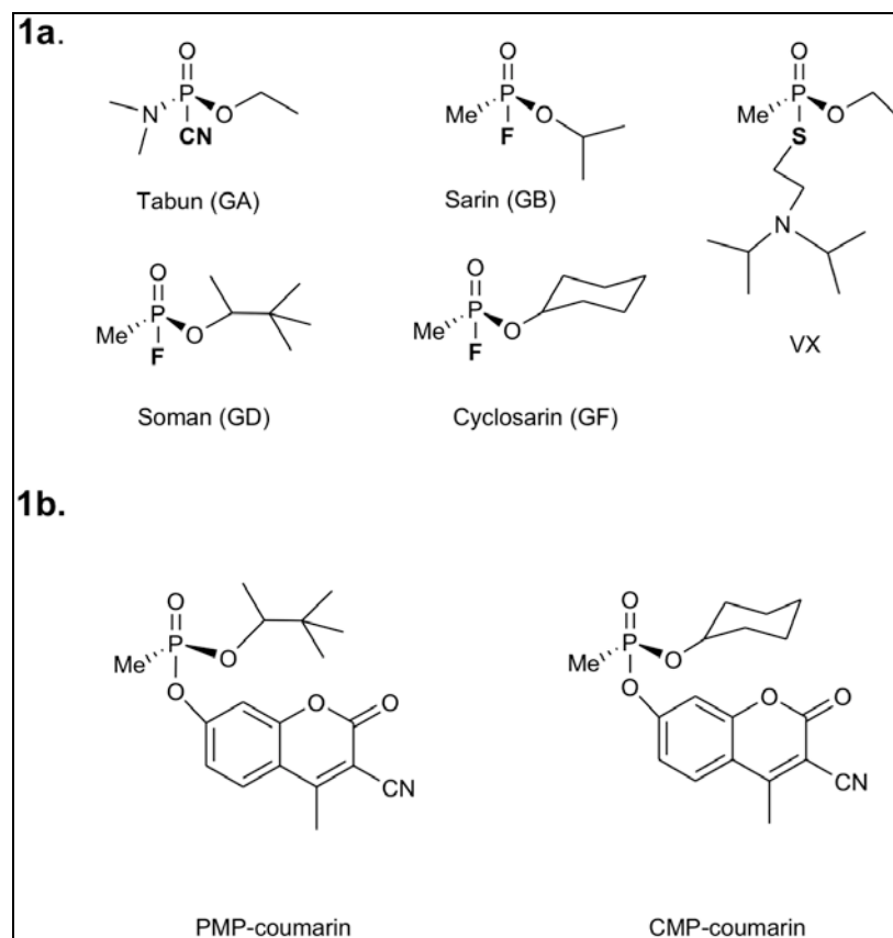
Figure 1. Nerve agents
