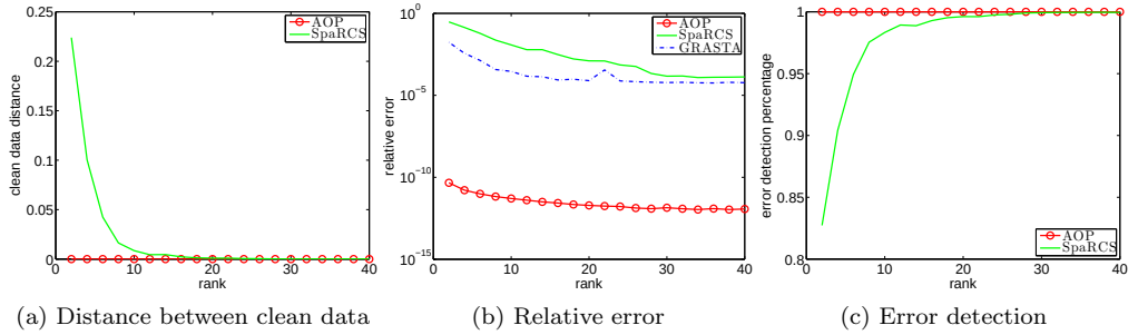
Figure 3: Algorithm comparison on corrupted data with different noise levels. (a) Distance between P_{\hat{\Omega}}(M_r) and P_{\hat{\Omega}}(M) vs rank, (b) Relative error vs rank, (c) Error location detection vs rank. AOP yields a remarkable improvement in reducing the relative error and finding the correct error locations compared with others.
