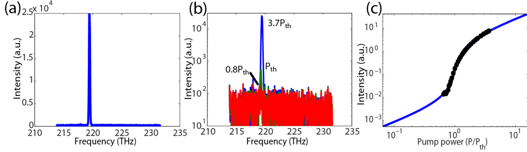
Figure 4.13. Lasing obtained from a band-edge mode (band D). (a) I show a lasing spectrum obtained at a peak pump power of 380 kW/cm 2 . (b) The semi-log scale pump-dependent spectra for the band-mode. (c) The L-L curve shows that the band-edge mode behaves the most classically, with a sharper threshold than both the \gamma - and \delta -defect modes. Since the exact nature of the bandedge mode is not known, the mode volume and quality factor of the mode cannot be used to find the Purcell enhancement and spontaneous emission coupling present in this mode. The threshold pump power for this device is 55kW/cm 2 of peak power.
