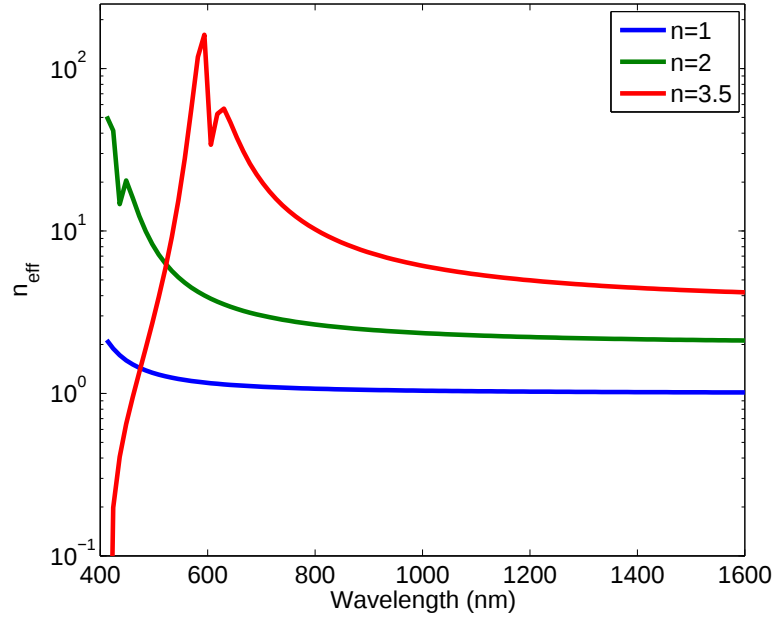
Figure 3.7. The effective index of a surface plasmon wave travelling between a silver and dielectric media with indices of refraction of n = 1 , n = 2 , and n = 3.5 .
