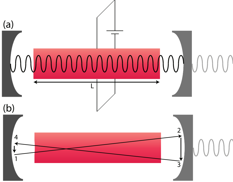
Figure 3.1. (a) A schematic of a Fabry-Pérot cavity laser. The laser consists of a semiconductor diode that acts as a gain material, and two mirrors on the two ends of the semiconductor. In practice, the edge of the laser chip serves as a mirror since the semiconductor can be cleaved to produce atomically smooth surfaces. (b) A simplified version of the movement of light within a laser cavity. As the light makes a round trip through the cavity, it gets amplified through the semiconductor, and attenuated at the mirrors as some light escapes the cavity. In one round trip, the light intensity must be equal for the laser to be self-sustaining.
