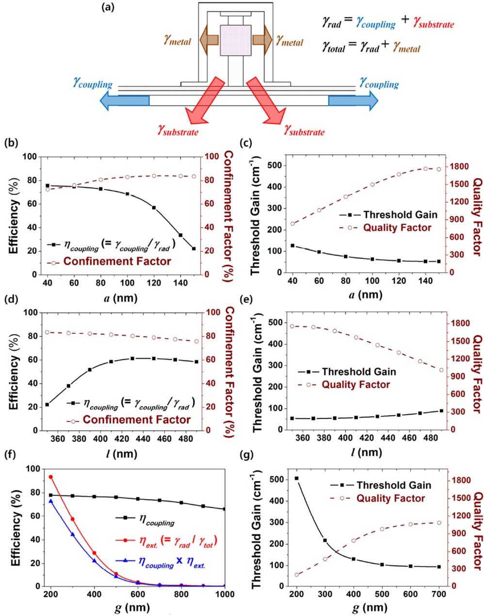
Figure 3.18. (a) Illustration showing the various energy loss paths from the cavity including metal and radiation losses. (b, c, d, e) Coupling efficiency ( \gamma_{\text{coupling}}/\gamma_{\text{rad}} ) to Si-waveguide, energy confinement factor into active region, threshold material gain coefficient for lasing, and cavity quality factor as a function of a and l , respectively, with b = 150 \text{ nm} and g = 600 \text{ nm} . (f, g) Coupling efficiency, total external efficiency, total energy efficiency to Si-waveguide, threshold material gain coefficient for lasing, and quality factor as a function of g for the optimal structure with a = 60 \text{ nm} , b = 150 \text{ nm} and l = 350 \text{ nm} .
