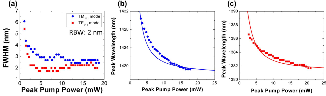
Figure 5.16. (a) The linewidth of both operating modes in the cylindrical nanopatch as a function of pumping power. (b,c) The wavelength shift of the laser wavelength as a function of pump power for the TM_{111} (b) and TE_{011} (c) modes.
