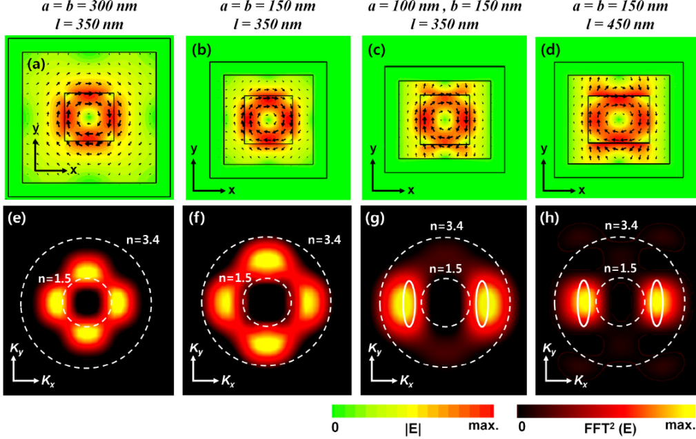
Figure 3.17. Electric field intensity profile (vector plot overlaid) and the Fourier transform of the electric field profile for (a, e) a = b = 300 nm and l = 350 nm, (b, f) a = b = 150 nm and l = 350 nm (c, g) a = 100 nm, b = 150 nm and l = 350 nm, and (d, h) a = b = 150 nm and l = 450 nm, respectively. Here, a , b and l are defined in Fig. 3.15c. The closed solid lines in (g) and (h) enclose the wavevectors that couple to the Si-waveguide.
