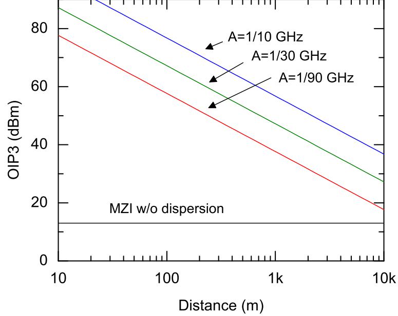
Figure 2.10: OIP3 for complementary linear-field discriminators for different slope values and fiber dispersion, assuming standard SMF, with D = -20 \text{ ps}^2/\text{km} , closely spaced tones around 2GHz, 5 mA of current per detector ( i_{dc} = 10\text{mA} ), 50 ohm impedance, and 0.5 amplitude bias, T = 0.25 .
