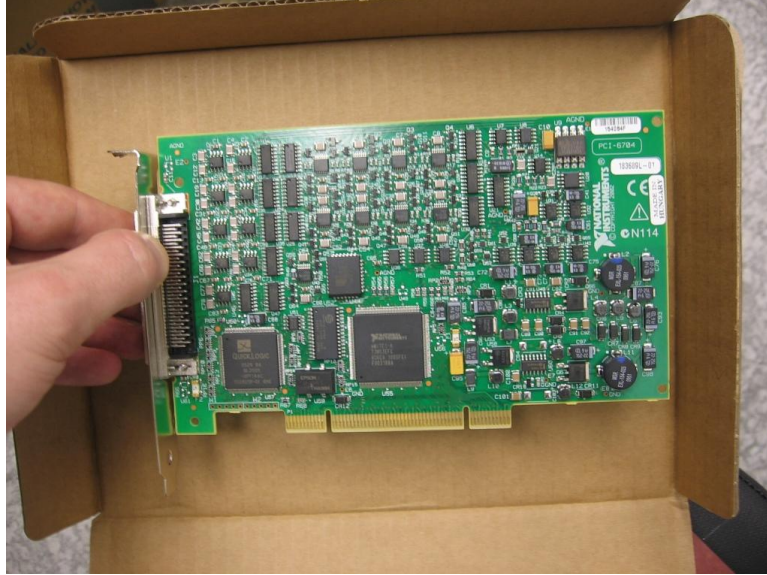
Figure 4.8: Photograph of National Instruments analog input/output card interface.
