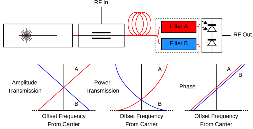
Figure 2.4: Ideal filter transfer functions for an optical PM or FM discriminator in a complementary linear-field demodulation scheme.
