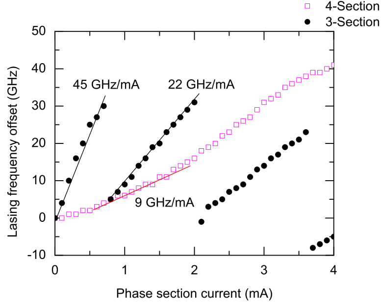
Figure 5.3: DC tuning measurement of DBR laser phase sections.
