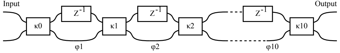
Figure 4.1: FIR lattice filter architecture
