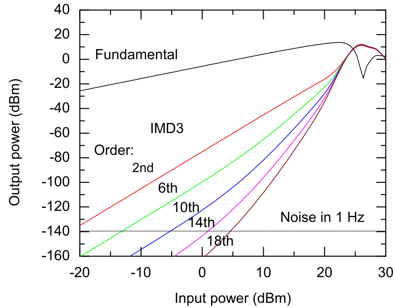
Figure 3.9: Link response versus input power for a 5 GHz PM-DD link using maximally linear filters of different order.
