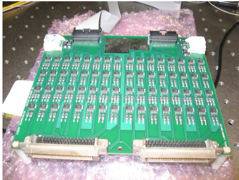
Figure 4.7: Photograph of current amplifier board to drive the chrome heaters on the tunable filters.
