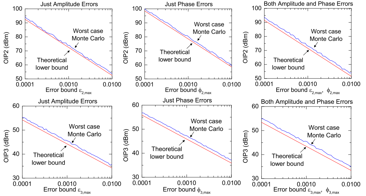
Figure 2.8: Monte Carlo simulation results to test the suitability of the derived bounds on the OIP2 and OIP3 . Each point is the worst case of 1000 trials with random errors, and is compared to the analytical bounds. We assume closely spaced tones around 2 GHz, 1/10 GHz slope, 5 mA of current per detector ( i_{dc} = 10\text{mA} ), 50 ohm impedance, and 0.5 amplitude bias, T = 0.25 . The analytical expression bounds the simulation within less than 2 dB.
