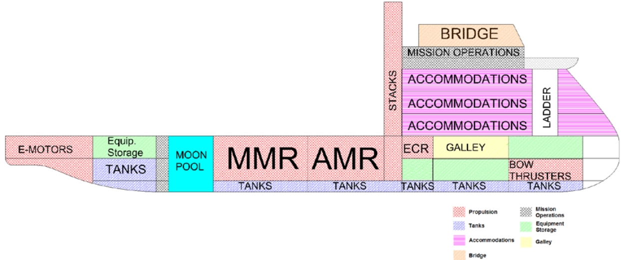
Figure 19: T-STAR Inboard Profile
