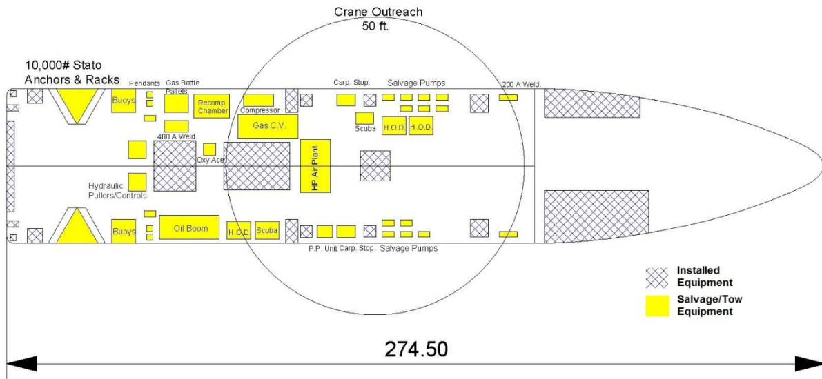
Figure 8: T-STAR Tow/Salvage Main Deck Layout
