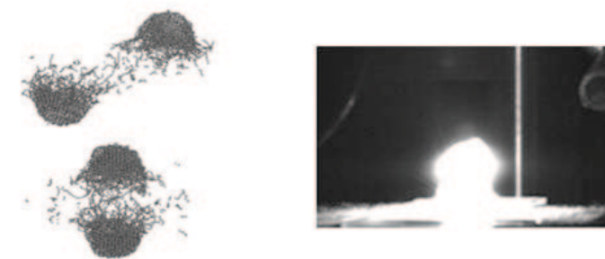
Figure 2. (left) Quantum mechanical simulations of two colliding nanodiamond particles, showing the significant spall and surface fragmentation. (right) Laser ignition of a conventional energetic material mixed with nanodiamonds.
