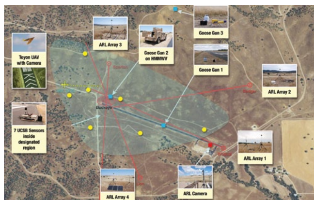
Persistent ISR scenario with networking and interoperability of two coalition networks: one sensor network with four acoustic arrays plus one fixed mounted camera and a second sensor network with seven low-cost unattended ground sensor (UGS) plus one unmanned aerial sensor (UAS) with visual camera onboard plus one UAS data harvester.
