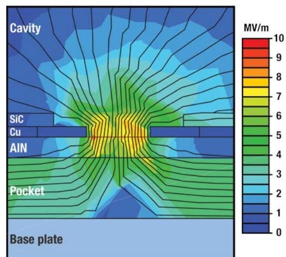
Electrostatic field simulation used to identify high electric field regions ( >7 MV/m) that could produce partial discharge and dielectric.
