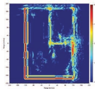
CAD model of complex room and resulting radar image generated using electromagnetic model data.
