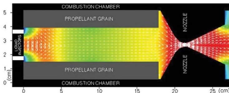
CFD modeling of a hybrid (HTPB-IRFNA) engine.
