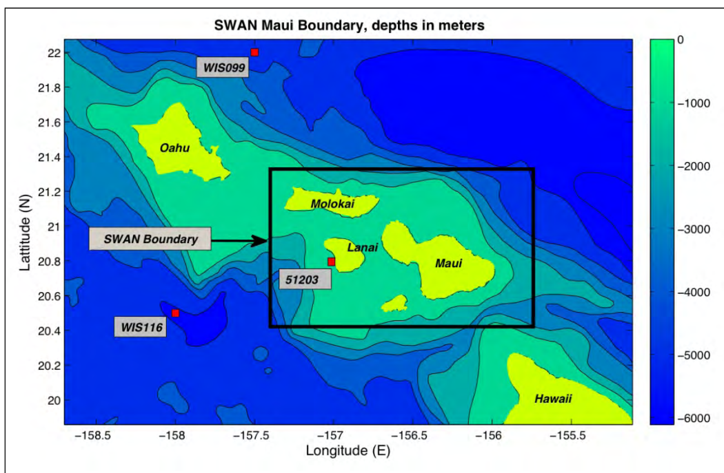
Figure 7.2. SWAN Maui domain (Sea Engineering, Inc. and Group 70 International 2009).
