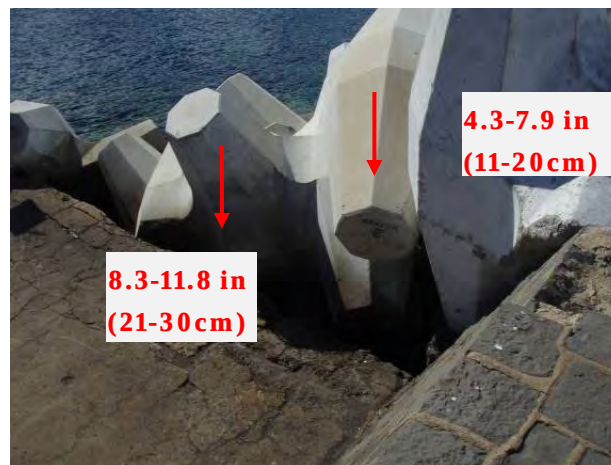
Figure 10.19. 2010 photo of harbor side tieback at Station -0+75. T-LiDAR measured settlement between 2007-2010 indicated for two armor units.
