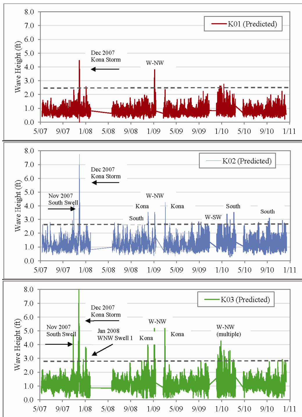
Figure 7.13. Time-series of KPWAVE-predicted wave height at K01, K02, and K03 stations.
