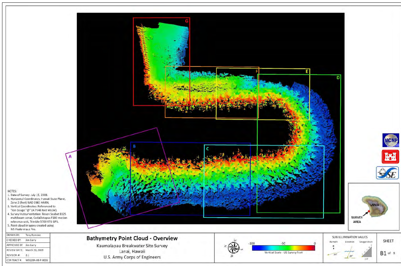
Figure 9.8. Bathymetry point cloud overview, and Section key, Kaomalapau Harbor breakwater (Sea Engineering, Inc. 2009).
