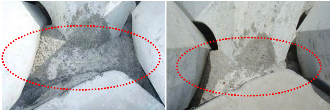
Figure 10.13. Grouted area along harbor side trunk at Station 1+80 (2007, left). Same area appears to have had some weathering and loss of grout (2009, right).
